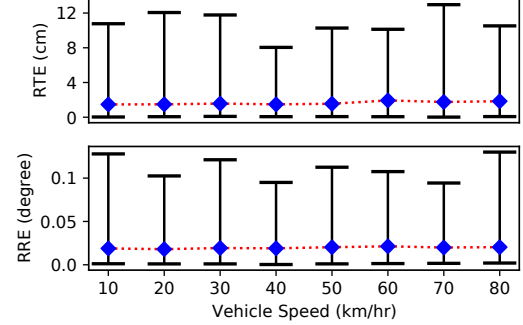
Figure 21: VRF’s accuracy as a function of vehicle speed.
