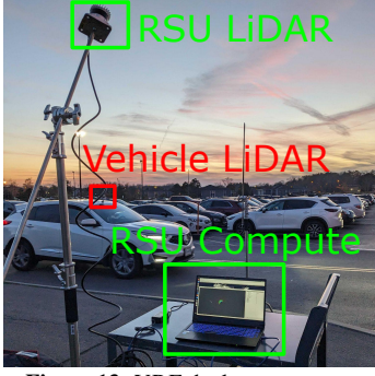
Figure 13: VRF deployment setup.
