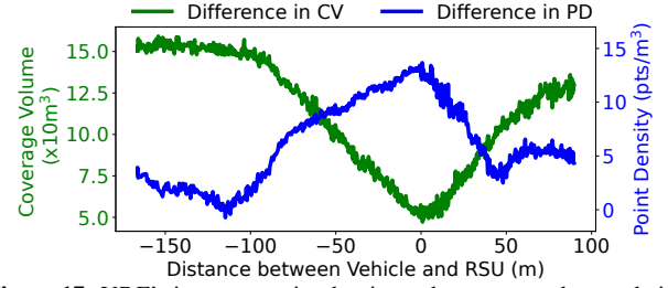
Figure 17: VRF’s improves point density and coverage volume relative to an un-fused vehicle point cloud. Both y-axes depict raw numbers (not percentages).
