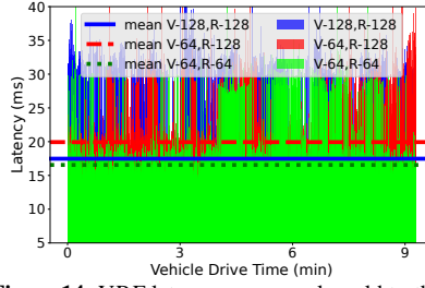
Figure 14: VRF latency on our real world tested with different LiDAR combinations.
